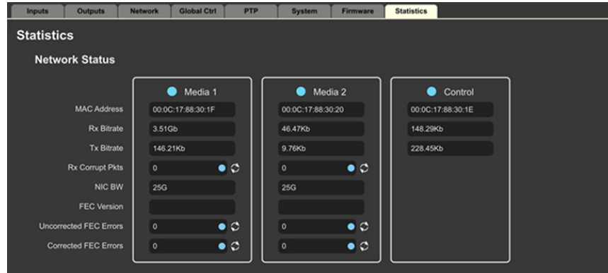
Figure 32. Statistics Tab
