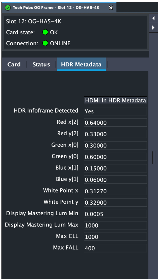
Figure 13. OG-HA5-4K HDR Metadata Tab Screen in DashBoard
