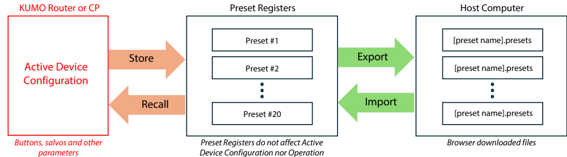
Figure 40. KUMO Presets Functional Block Diagram
