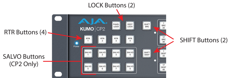
Figure 67. KUMO CP Function Buttons
