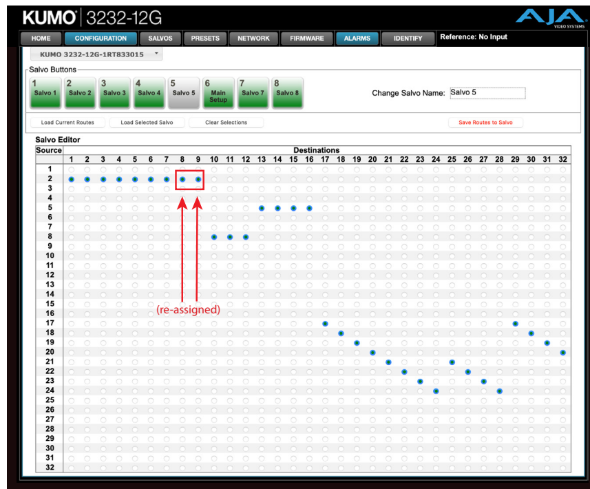
Figure 34. Result of the example Salvo 2 Take
