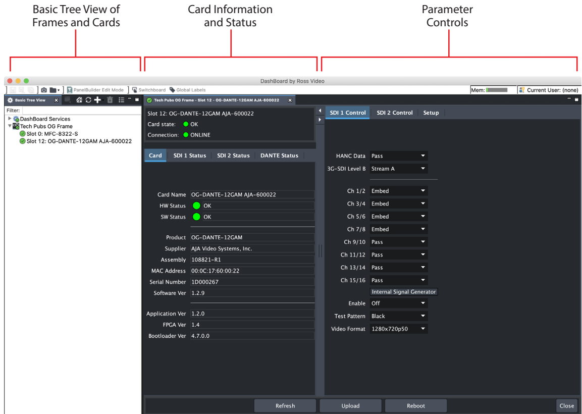
Figure 10. Main Sections of the DashBoard User Interface
