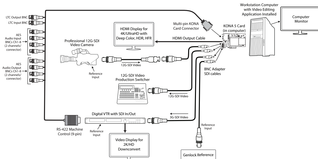
Figure 12. Typical KONA 5 System Connections, 4K Mode
