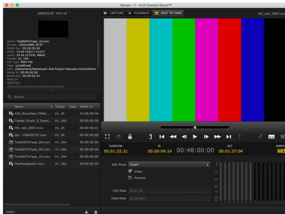
Figure 14. Edit-To-Tape Tab
