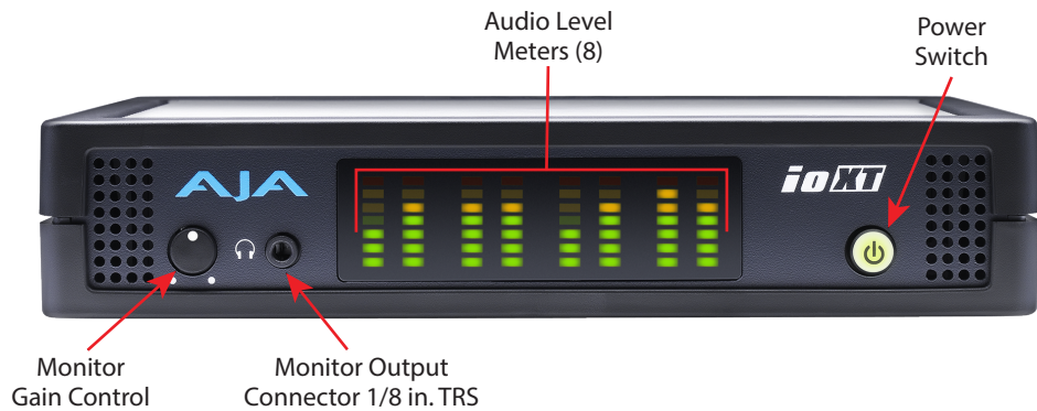
Figure 4. Io XT Front Panel Controls and Indicators
