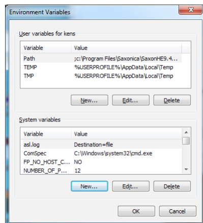
Figure 16. Environment Variables Screen
