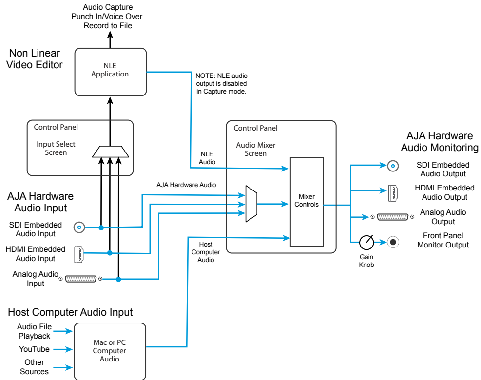
Figure 16. lo 4K in 4K Mode Audio Monitoring Routing Diagram
