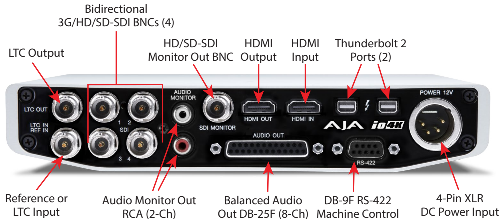
Figure 2. lo 4K Rear Connectors
