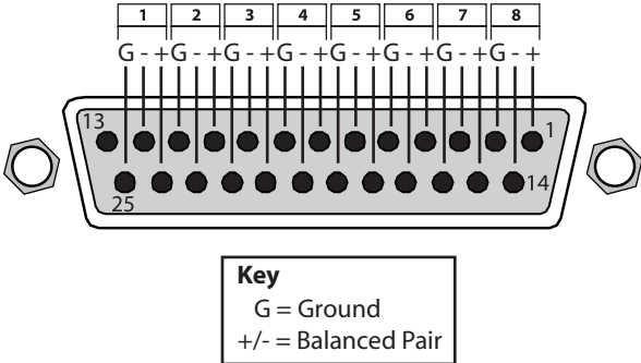
Figure 24. DB-25 Analog Audio Connector Pinouts
