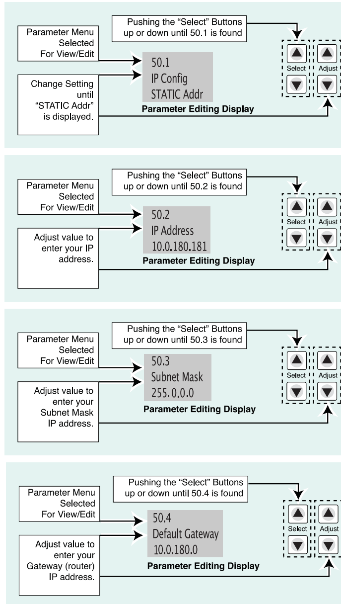
Configuring Ki Pro Mini with a Static IP Address
